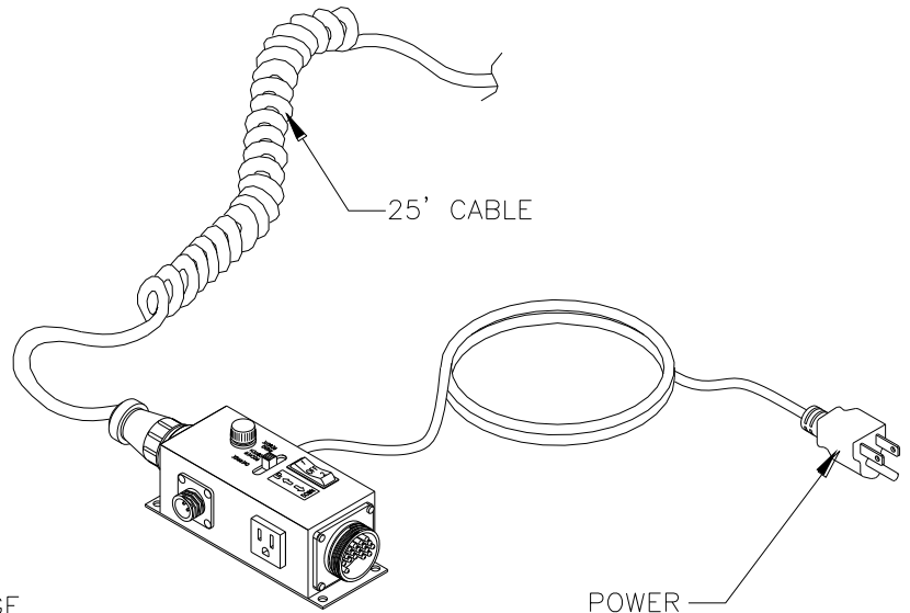
EXTERNAL JUNCTION BOX
